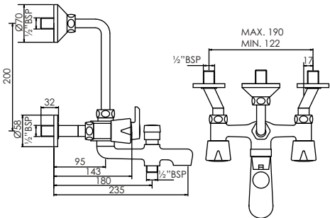
Wall Mixer 3 in 1 with Bend Pipe T1823C
