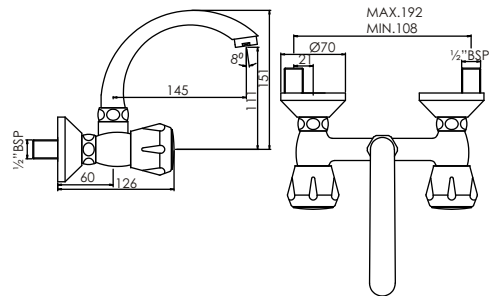
Sink Mixer with Swivel Spout T1620C
