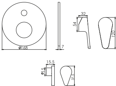
3 inlet Single Lever Concealed Diverter T0439C Upper Chrome Trims #To be fitted with Concealed Diverter Body T0066C
