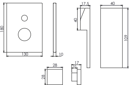
Single Lever Concealed Diverter T2640C4 Upper Chrome Trims #To be fitted with Concealed Diverter Body T2636C0
