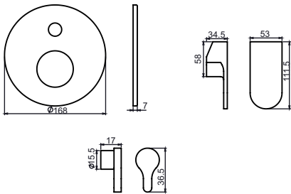
3 Inlet Single Lever T0139C Upper Chrome Trims #To be fitted with Concealed Diverter Body T0066C
