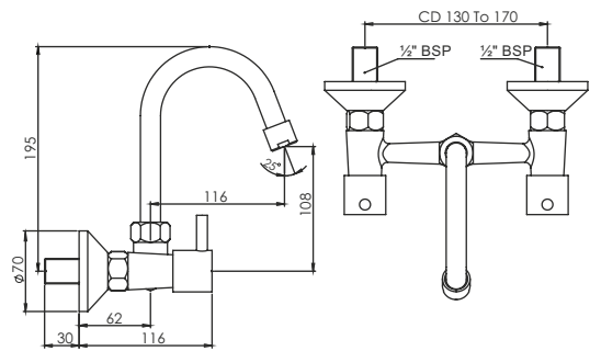
Wall Mixer 2 in 1 with Bend Pipe T2921C
