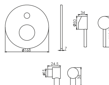
3 Inlet Single Concealed Divertor
