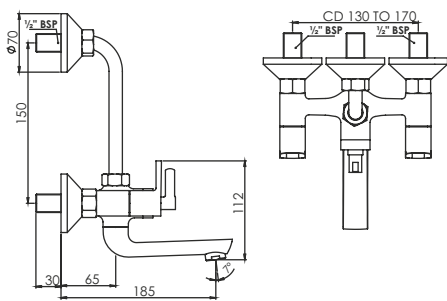
Wall Mixer 2 in 1 with Bend Pipe T3421C
