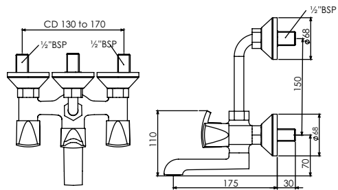
Wall Mixer 2 in 1 with Bend pipe T2521C
