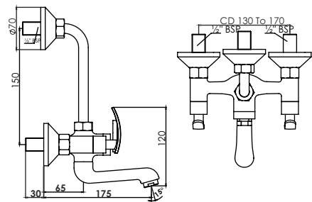
Wall Mixer 2 in 1 with Bend pipe T3021C
