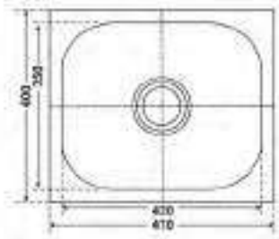
Elegance SS304 Kitchen Sink with Waste Coupling Outer Dimensions : 470x400mm Bowl Dimensions : 420x350x180mm K0201 Satin Finish
