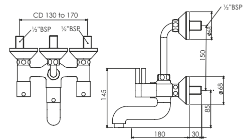
Wall Mixer 2 in 1 with Bend Pipe T1321C
