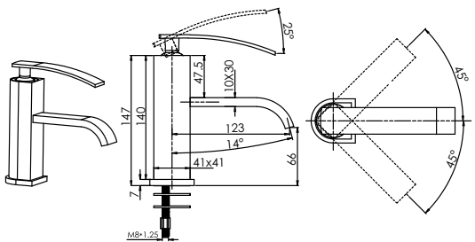
Single Lever Basin Mixer T3645C
