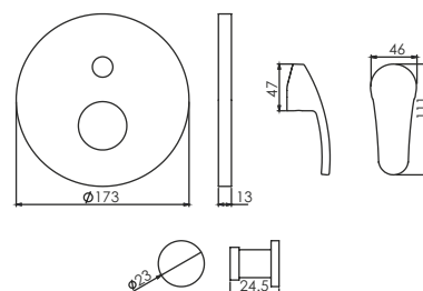
High Flow Single Lever Concealed Diverter T0778C Upper Chrome Trims #To be fitted with Concealed Diverter Body T0078C
