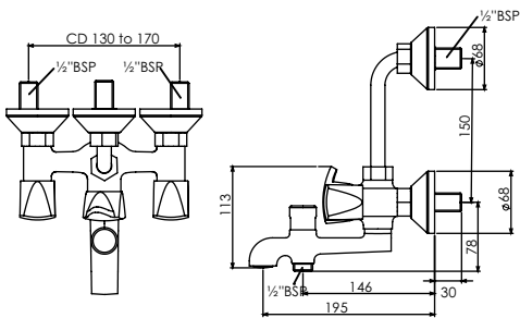
Wall Mixer 3 in 1 with Bend pipe T2523C
