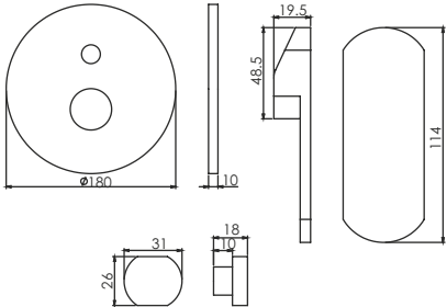
Single Lever Concealed Diverter T2640C3 Upper Chrome Trims #To be fitted with Concealed Diverter Body T2636C0
