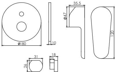
Single Lever Concealed Diverter T2640C1 Upper Chrome Trims #To be fitted with Concealed Diverter Body T2636C0
