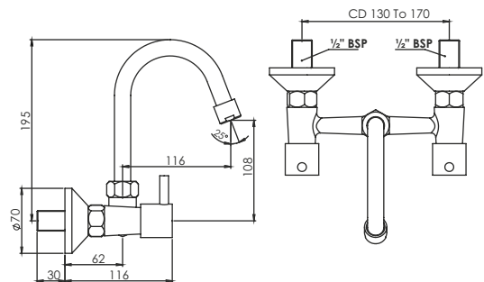
Sink Mixer with Cast Spout T2976C
