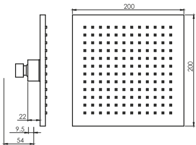
Optima Plus Rain Shower Square O1740C 200mm
