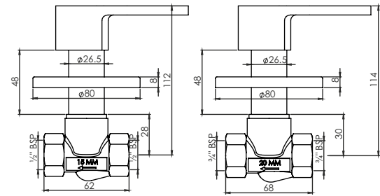
Concealed Stop Cock T2613C2 15mm T2615C2 20mm
