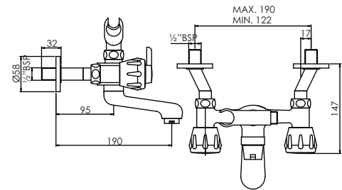
Wall Mixer 2 in 1 with Crutch T1722C
