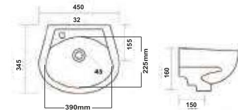
Flora Dimensions : 450x345x160mm P1315PW Basin
