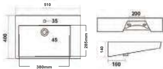
Slide Dimensions : 510x400x140mm P4715PW Basin
