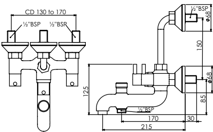
Wall Mixer 3 in 1 with Bend Pipe T2423C
