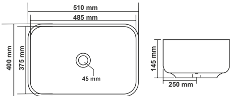
Omega Recta Dimensions : 510x400x145mm P7312PW
