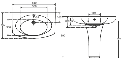
Grande Dimensions : 630x460x180mm P6215PW Basin P6216PW Full Pedestal
