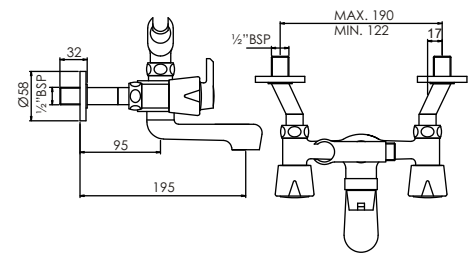
Wall Mixer 2 in 1 with Crutch T1822C
