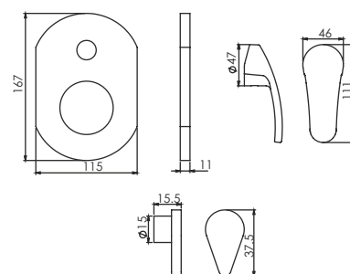
3 Inlet Single Lever Concealed Diverter T0739C Upper Chrome Trims #To be fitted with Concealed Diverter Body T0066C
