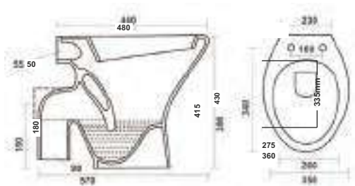
Pearl EWC S Trap / P Trap Dimensions : 570x350x390mm P0347PW S Trap P0346PW P Trap
