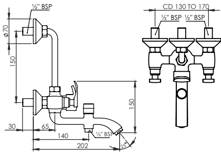
Wall Mixer 3 in 1 with Bend Pipe T3123C
