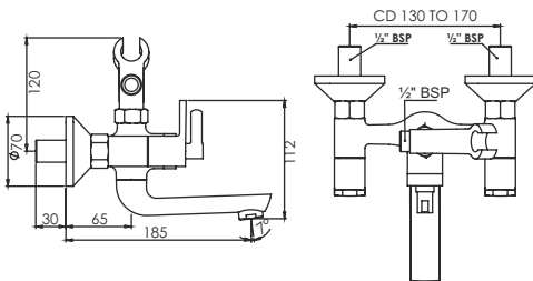
Wall Mixer 2 in 1 with Crutch T3422C
