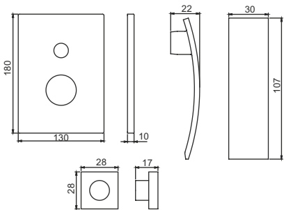
Single Lever Concealed Diverter T3640C Upper Chrome Trims #To be fitted with Concealed Diverter Body T2636C5
