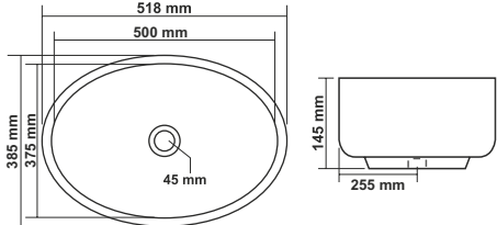
Omega Oval Dimensions : 515x385x145mm P7312PW
