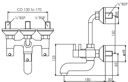
Wall Mixer 2 in 1 with Bend Pipe T2421C
