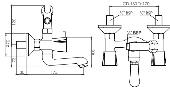
Wall Mixer 2 in 1 with Crutch T2822C
