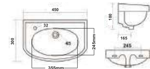
Iris Dimensions : 450x300x180mm P1415PW Basin
