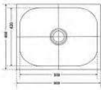
Elegance SS304 Kitchen Sink with Waste Coupling Outer Dimensions : 600x470mm Bowl Dimensions : 550x420x220mm K0203 Satin Finish
