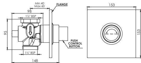
Cosmo Single Flush Valve with Square Flange T2375C 40mm
