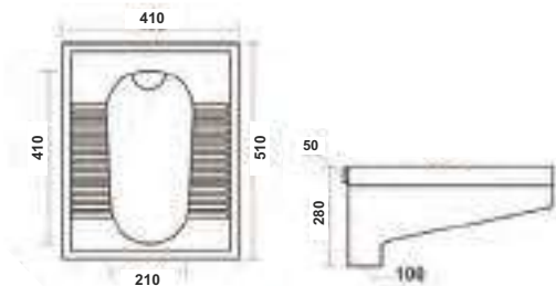
Ruby Orissa Pan(Open Rim) Dimensions : 510x410x250mm P0459PW OP20 # Also available in ISI
