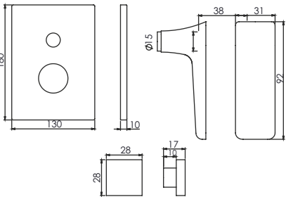
Single Lever Concealed Diverter T2640C5 Upper Chrome Trims #To be fitted with Concealed Diverter Body T2636C5
