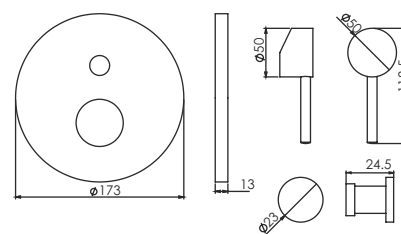
High Flow Single Concealed Divertor
