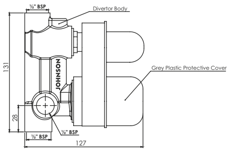
Single Lever Concealed Diverter Body T2636C0 Suitable For Elite 1000, 2000, 3000, 4000 & Altis Single Lever Concealed Diverter
