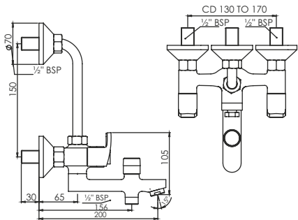
Wall Mixer 3 in 1 with Bend Pipe T0723C
