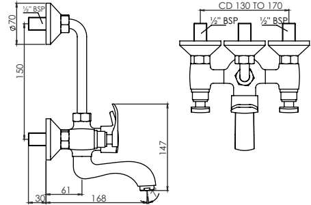
Wall Mixer 2 in 1 with Bend Pipe T3121C
