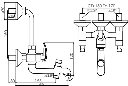
Wall Mixer 3 in 1 with Bend pipe T3023C
