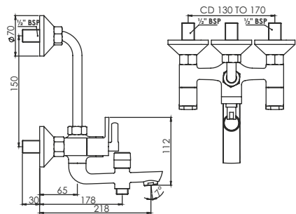
Wall Mixer 3 in 1 with Bend Pipe T3423C
