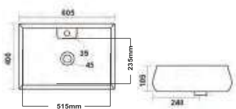
Altis Dimensions : 605x400x105mm P5312PW
