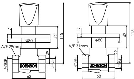
Concealed Stop Cock with Body T2513C 15mm T2515C 20mm
