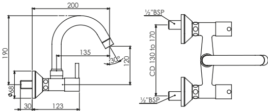
Sink Mixer with Swivel Spout T1320C
