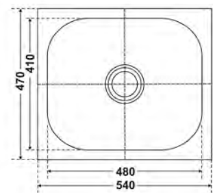
Elegance SS304 Kitchen Sink with Waste Coupling Outer Dimensions : 540x470mm Bowl Dimensions : 480x410x200mm K0202 Satin Finish
