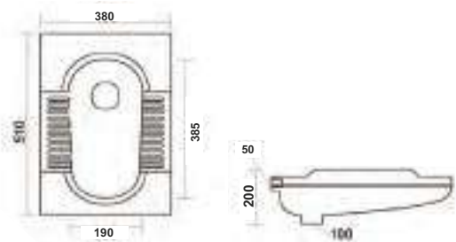
Ruby Arab Pan(Open Rim) Dimensions : 510x380x200mm P0442PW AP20
