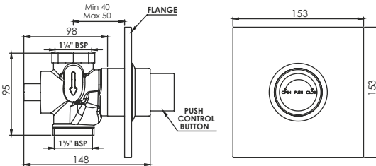
Cosmo Single Flush Valve with Square Flange T2373C 32mm
