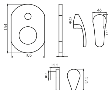
Single Lever Concealed Diverter T0740C Upper Chrome Trims #To be fitted with Concealed Diverter Body T0036C
