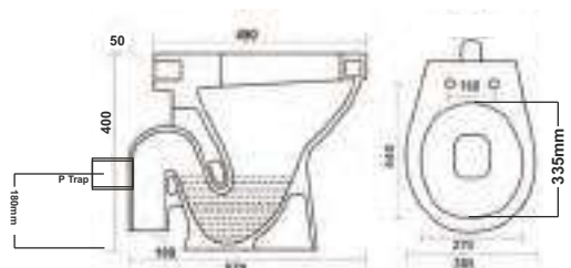
Ruby EWC S Trap / P Trap Dimensions : 570x365x400mm P0447PW S Trap P0446PW P Trap # Also available in ISI
