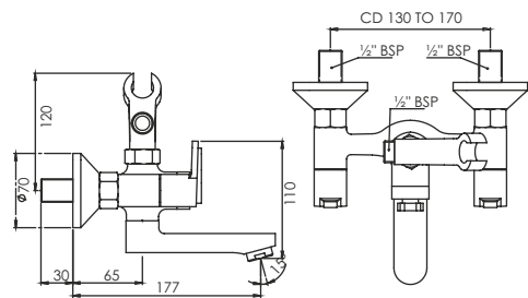
Wall Mixer 2 in 1 with Crutch T0622C
