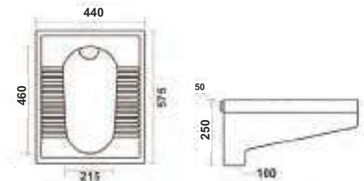
Ruby Orissa Pan(Open Rim) Dimensions : 575x440x250mm P0461PW OP23 # Also available in ISI
