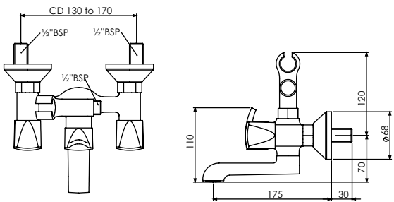
Wall Mixer 2 in 1 with Crutch T2522C
