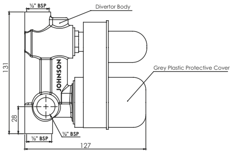
Single Lever Concealed Diverter Body T2636C5 Suitable For Elite 5000 & Omega Single Lever Concealed Diverter
