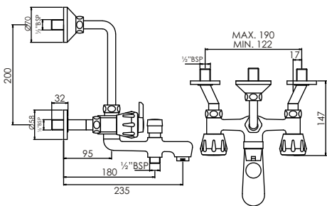
Wall Mixer 3 in 1 with Bend Pipe T1723C
