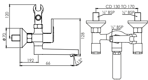
Wall Mixer 2 in 1 with Crutch T3222C
