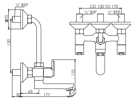
Wall Mixer 2 in 1 with Bend Pipe T0621C
