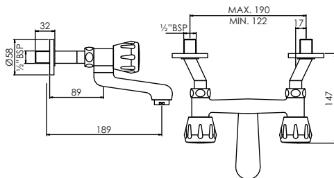
Wall Mixer with Non Telephonic T1724C
