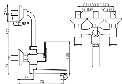
Wall Mixer 2 in 1 with Bend Pipe T3221C
