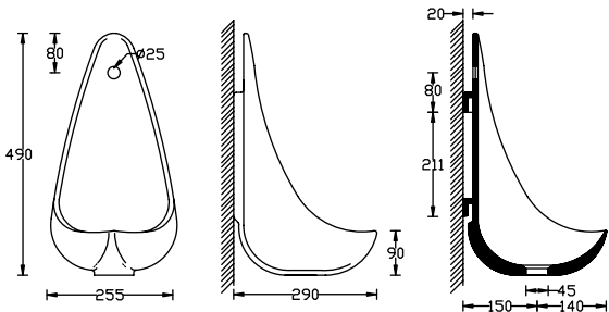
Kito with Spreader Dimensions : 290x255x490mm P2719PW Kito Urinal
