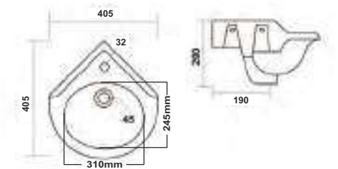
Ruby Corner Dimensions : 405x405x200mm P0445PW Basin
