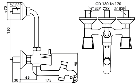
Wall Mixer 3 in 1 with Bend pipe T2823C
