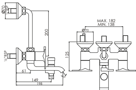
Wall Mixer 3 in 1 with Bend Pipe T0223C
