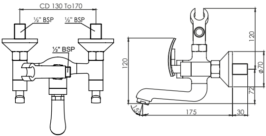
Wall Mixer 2 in 1 with Crutch T3022C
