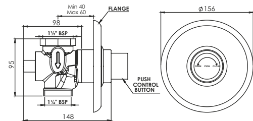
Cosmo Single Flush Valve with Round Flange T2357C 40mm
