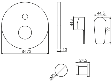
Single Lever Concealed Diverter T3478C Upper Chrome Trims #To be fitted with Concealed Diverter Body T0078C
