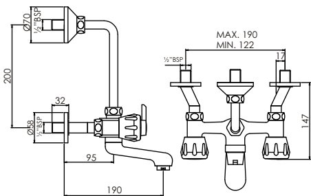
Wall Mixer 2 in 1 with Bend Pipe T1721C
