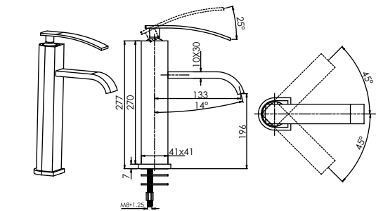
Single Lever Tall Basin Mixer T3646C
