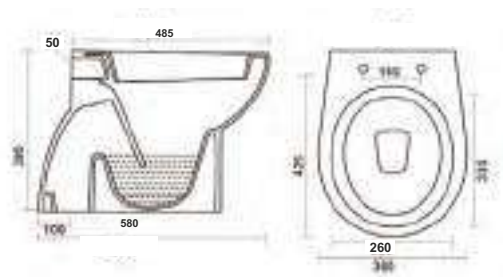
Ruby Concealed Trap EWC S Trap Dimensions : 580x360x395mm P0448PW S Trap
