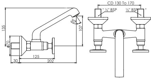
Sink Mixer with Swivel Spout T3520C
