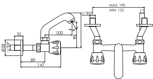
Sink Mixer with Swivel Spout T1720C
