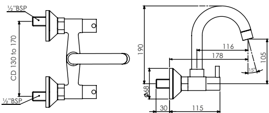
Sink Mixer with Swivel Spout T2420C
