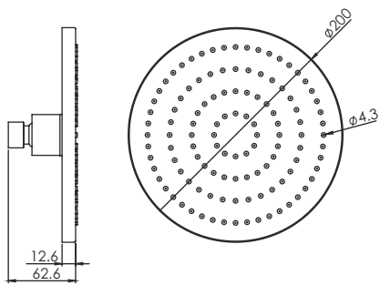
Optima Plus Air Rain Shower Round O1739C 200mm
