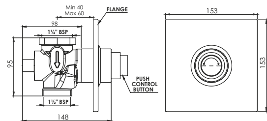
Cosmo Dual Flush Valve with Square Flange T2376C 40mm
