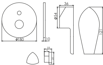
Single Lever Concealed Diverter T2340C2 Upper Chrome Trims #To be fitted with Concealed Diverter Body T2636C0
