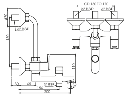
Wall Mixer 3 in 1 with Bend Pipe T0623C
