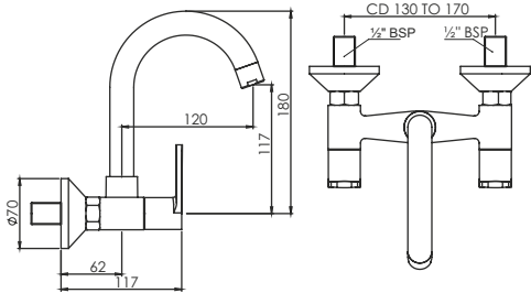
Sink Cock Wall Mounted T3218C
