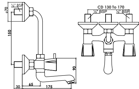
Wall Mixer 2 in 1 with Bend pipe T2821C
