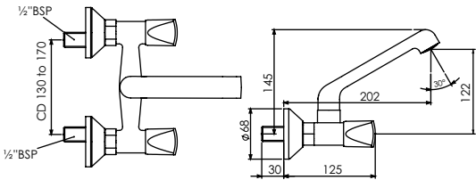
Sink Mixer with Swivel Spout T2520C
