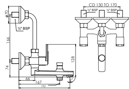
Wall Mixer 3 in 1 with Bend Pipe T3223C
