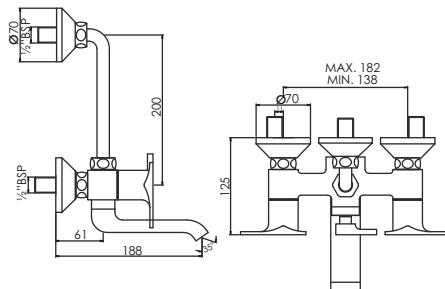
Wall Mixer 2 in 1 with Bend Pipe T0221C
