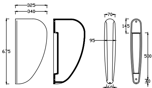
Flair Division Plate For Urinals Dimensions : 320x95x675mm P2811PW
