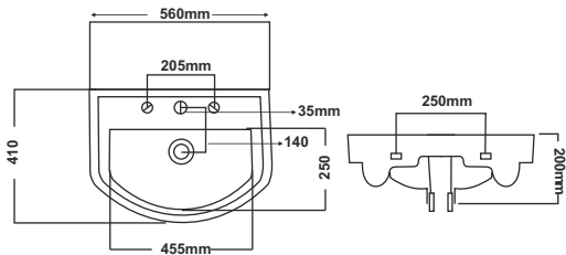
Daisy Dimensions : 560x410x200mm P1115PW Basin P1117PW Half Pedestal P1116PW Full Pedestal
